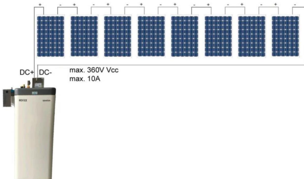
Figure 1: wiring schematic of PV Panels
